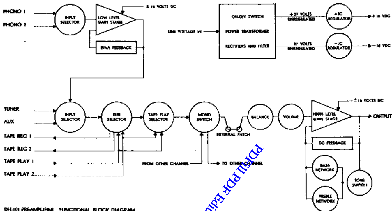
DH-101 PREAMPLIFIER FUNCTIONAL BLOCK DIAGRAM
