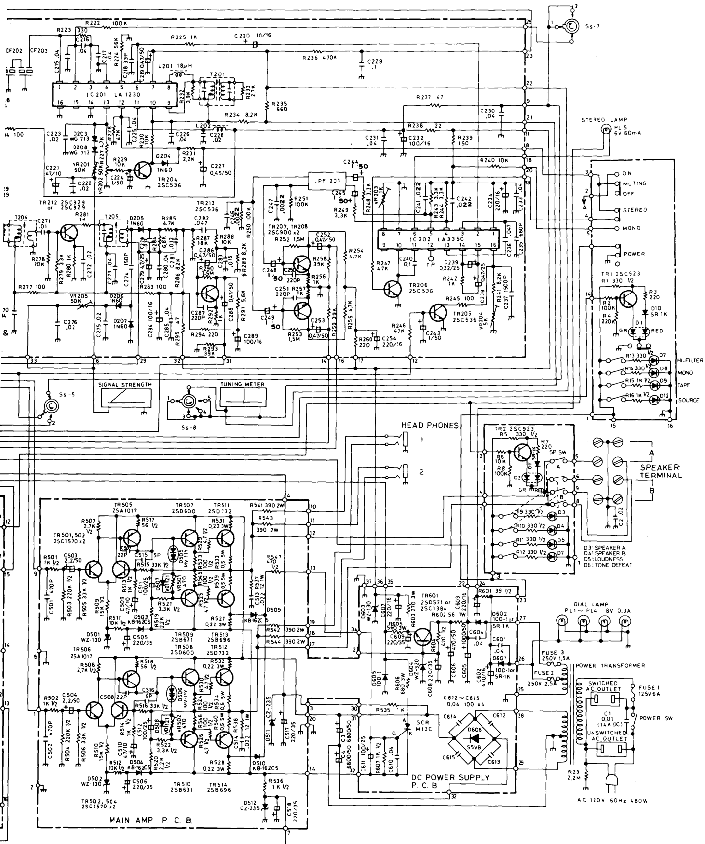
SCHMATIC DIAGRAM Concept 4.5
